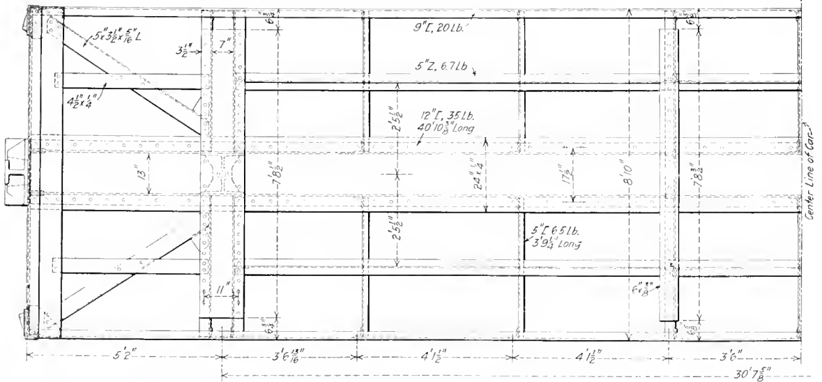
Steel Underframe for Santa Fe Stock Cars
